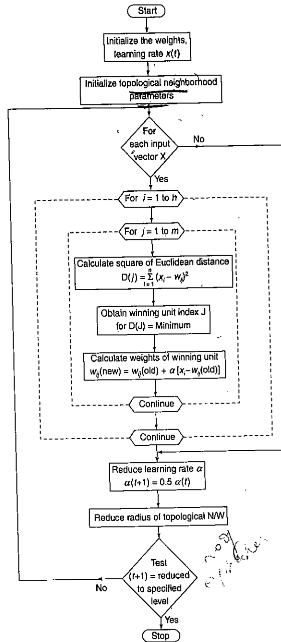
Figure 5-11 Flowchart for training process of KSOFM.
