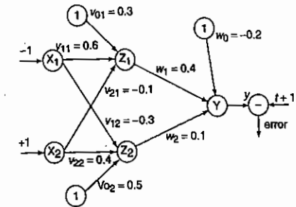
Figure 13 Network.
