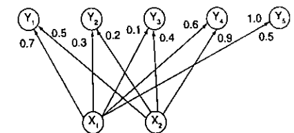
Figure 11 KSOFM net.
