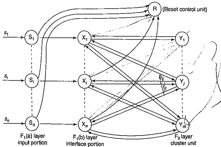
Figure 5-22 Basic architecture of ART 1.
