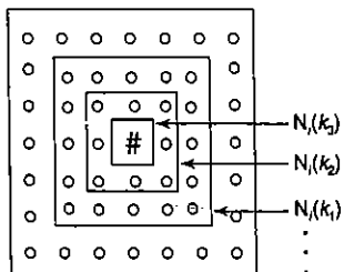
Figure 5-8 Rectangular grid.
