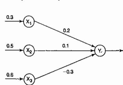
Figure 1 Neural net.
