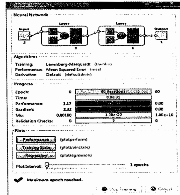
Figure 16-23 Neural Network Training Tool for the given input and output pairs.
